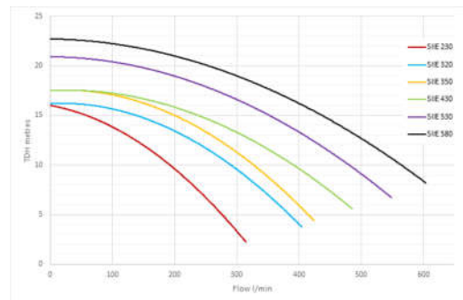
SUPER II ECO PUMP PERFORMANCE
